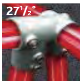
Type 185 27 \frac{1}{2} ° Eeyes Fitting D
